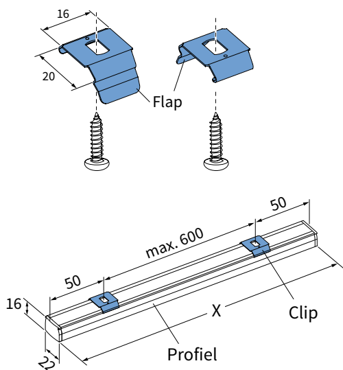
Standaard profiel 13 [mm] x 20 [mm] Clip
